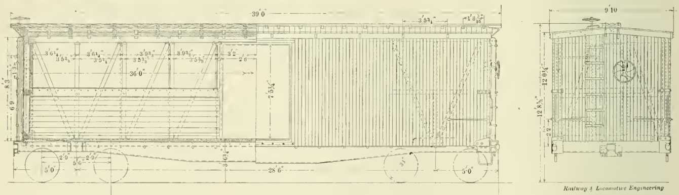
PENNSYLVANIA PRESSED STEEL CAR.
